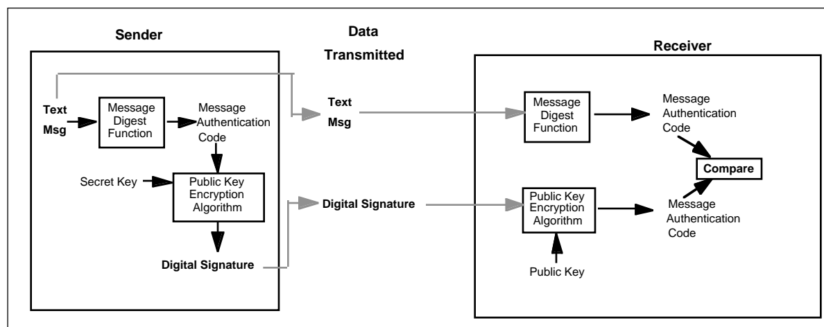
Figure 30: Public Key Digital Signatures
