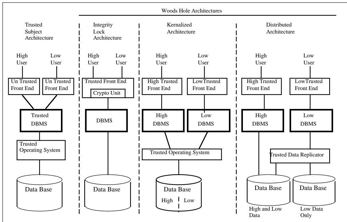
Figure 26: MLS DBMS Schemes
