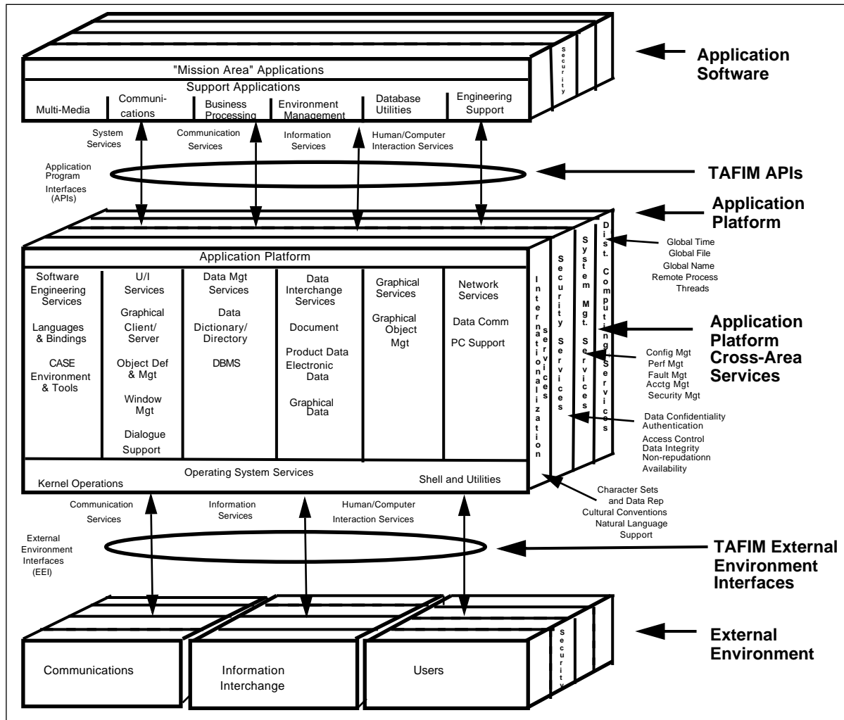
Figure 35: DoD TAFIM Technical Reference Model
