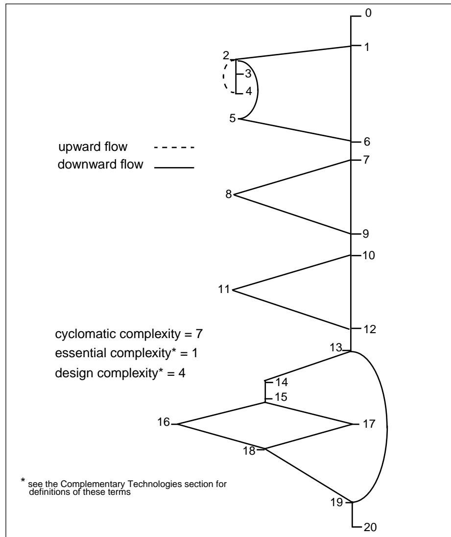
Figure 11: Connected Graph of a Simple Program
