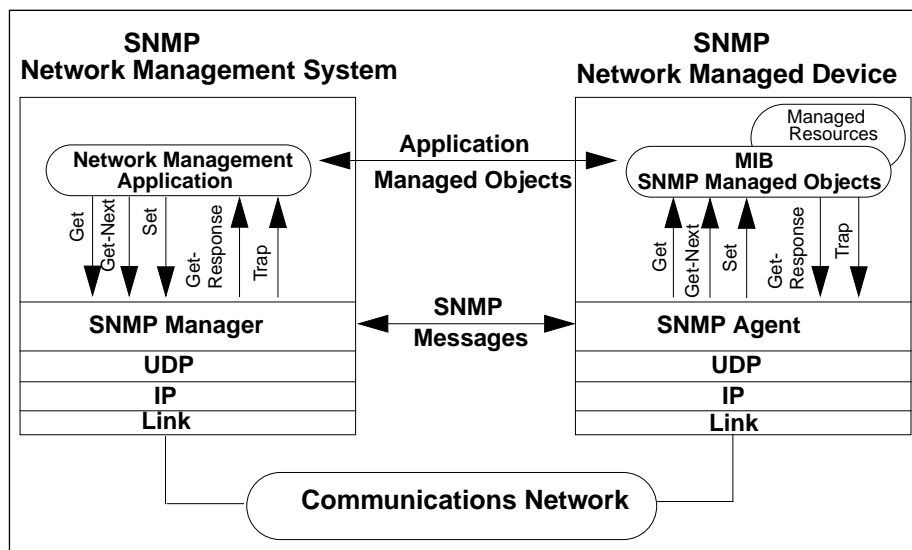
Figure 33: The SNMPv1 Architecture [Lake 96]
