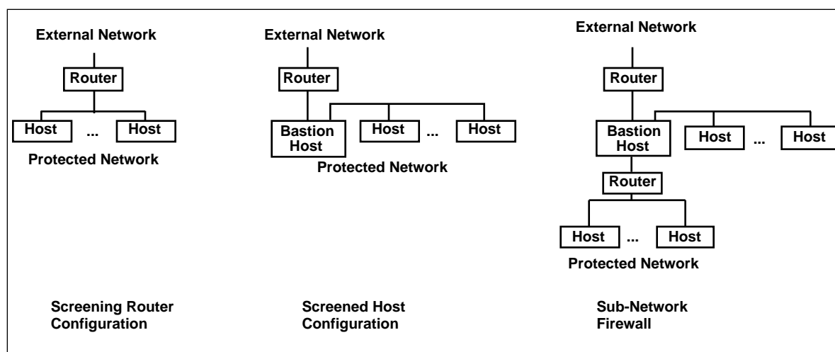
Figure 18: Firewall Configurations
