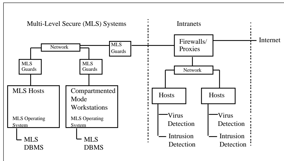
Figure 10: Computer System Security in C4I Systems
